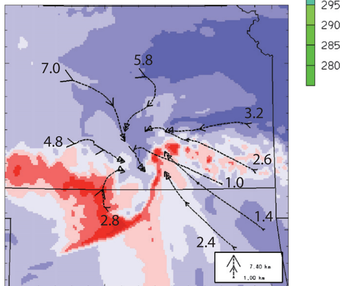
d) 3 km trajectories, 700 hPa \theta_e
