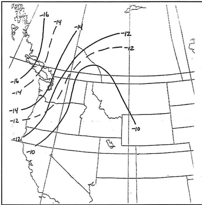
Fig. 22. Average 500-mb temperatures ( ^{\circ}\text{C} ) at 1200 UTC (dashed) and 0000 UTC (solid) during Pattern A SSWs in Washington and Oregon.
