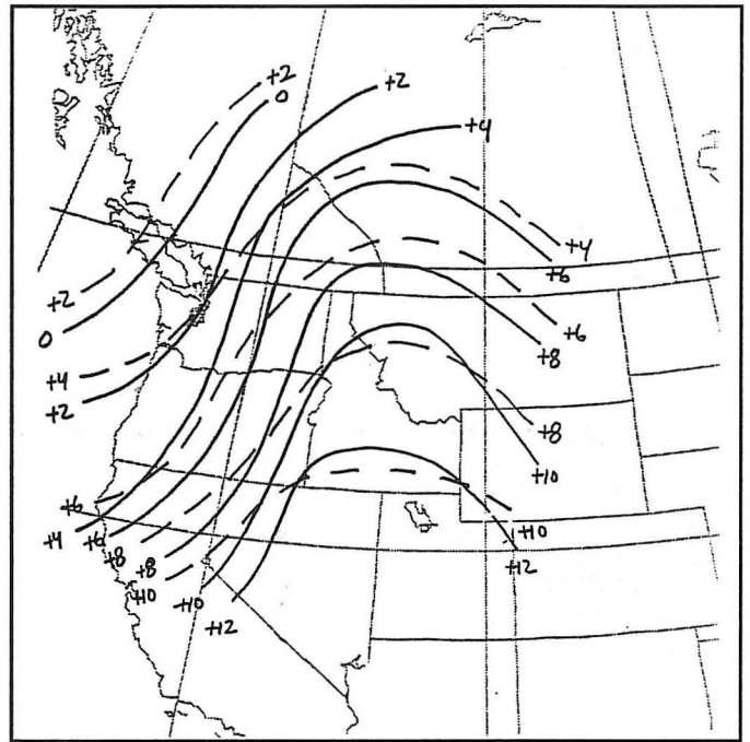
Fig. 23. Average 700-mb temperatures ( ^{\circ}\text{C} ) at 1200 UTC (dashed) and 0000 UTC (solid) during Pattern A SSWs in Washington and Oregon.
