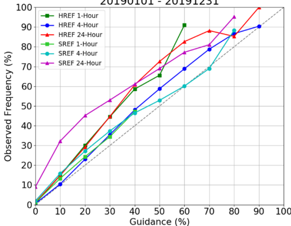
Figure 2: Comparison of the (a) performance and (b) reliability of the HREF and SREF Calibrated Thunder 1-hour, 4-hour, and 24-hour forecasts from 1 January 2019 – 1 January 2020.
