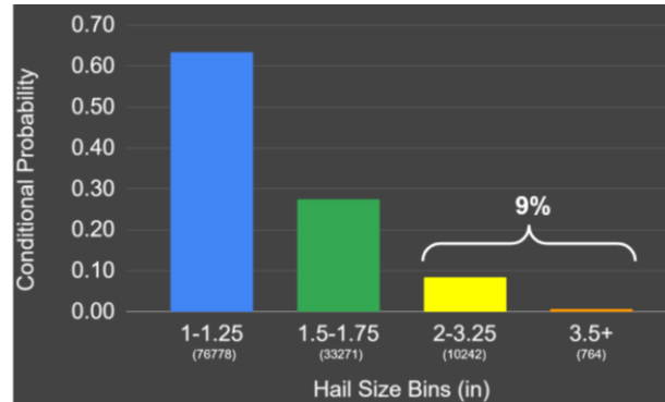
Figure 5. Hail report bins utilized in this study: 1-1.25" (blue), 1.5-1.75" (green), 2-3.25" (yellow), and 3.5"+ (orange). The conditional probability of a severe report falling into each of these bins is provided on the y-axis, and the sample size per bin is denoted in parentheses. Note that only 9% of all severe hail grid hours from 2003-2020 were significant severe (i.e., 2"+).
