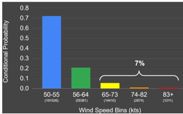
Figure 3. Wind report bins utilized in this study: 50-55 kts (blue), 56-64 kts (green), 65-73 kts (yellow), 74-82 kts (orange), and 83+ kts (red). The conditional probability of a severe report falling into each of these bins is provided on the y-axis, and the sample size per bin is denoted in parentheses. Note that only 7% of all severe wind grid hours from 2003-2020 were significant severe (i.e., 65+ kts).
