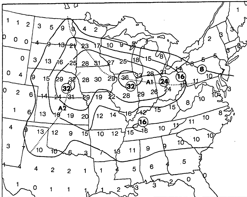
FIG. 12. Total number of northwest flow outbreaks occurring in 2^\circ Marsden squares for the period 1962–77. A1 and A2 high-frequency axes are indicated by dotted lines (from Johns, 1982b).
