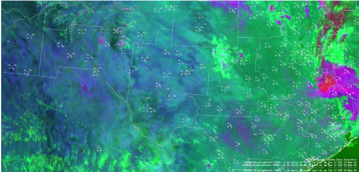
Figure 29: The Moisture Gradient Convective RGB sandwich from 1726 Z on 23 May 2023.
