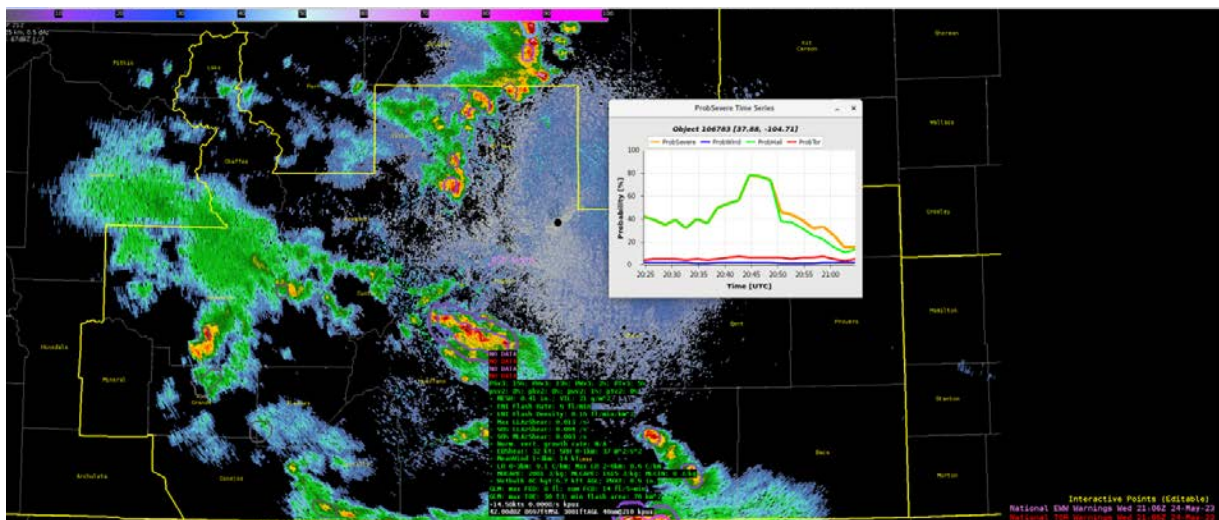
Figure 25: ProbSevere all hazards overlaid on KPUX base reflectivity from 2042 Z on 14 June 2023.
